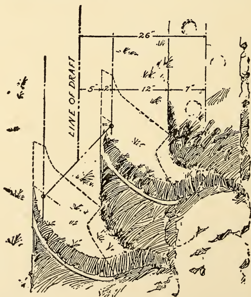
TRUE LINE OF DRAFT-TWO 14" BOTTOMS
